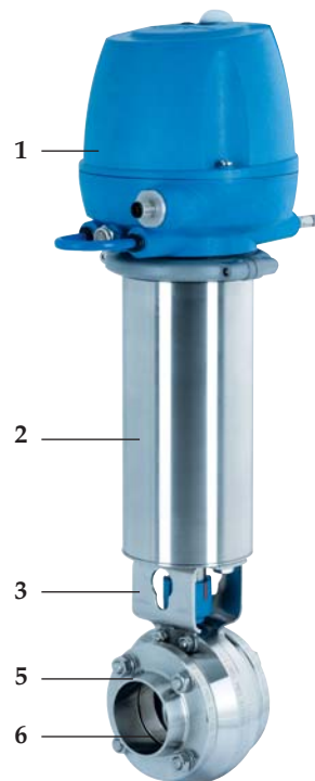
Type VV with pneumatic actuator
